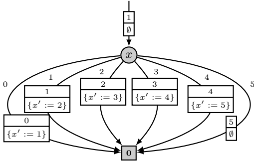
Figure 4: EVMDD over \mathcal{N} \otimes \mathcal{F} for cost function x + 1 and conditional effect x' := x + 1 combined. Edge labels have their \mathcal{N} -part on top, and their \mathcal{F} -part at the bottom.
