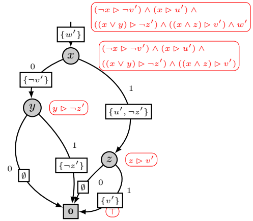
Figure 6: EVMDD for (\neg x \triangleright \neg v') \wedge (x \triangleright u') \wedge ((x \vee y) \triangleright \neg z') \wedge ((x \wedge z) \triangleright v') \wedge w' .
