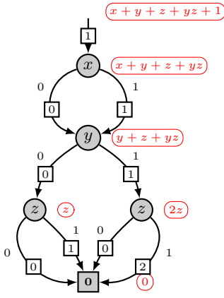
Figure 5: EVMDD for x + y + z + yz + 1 .
