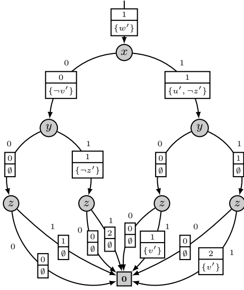
Figure 7: EVMDD for x + y + z + yz + 1 and (\neg x \triangleright \neg v') \wedge (x \triangleright u') \wedge ((x \vee y) \triangleright \neg z') \wedge ((x \wedge z) \triangleright v') \wedge w' combined.
