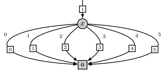
Figure 2: EVMDD over \mathcal{N} for cost function x + 1 .
